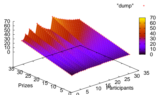
Figure 2: Average number of coin-flips for a game for a number of participants and prizes
